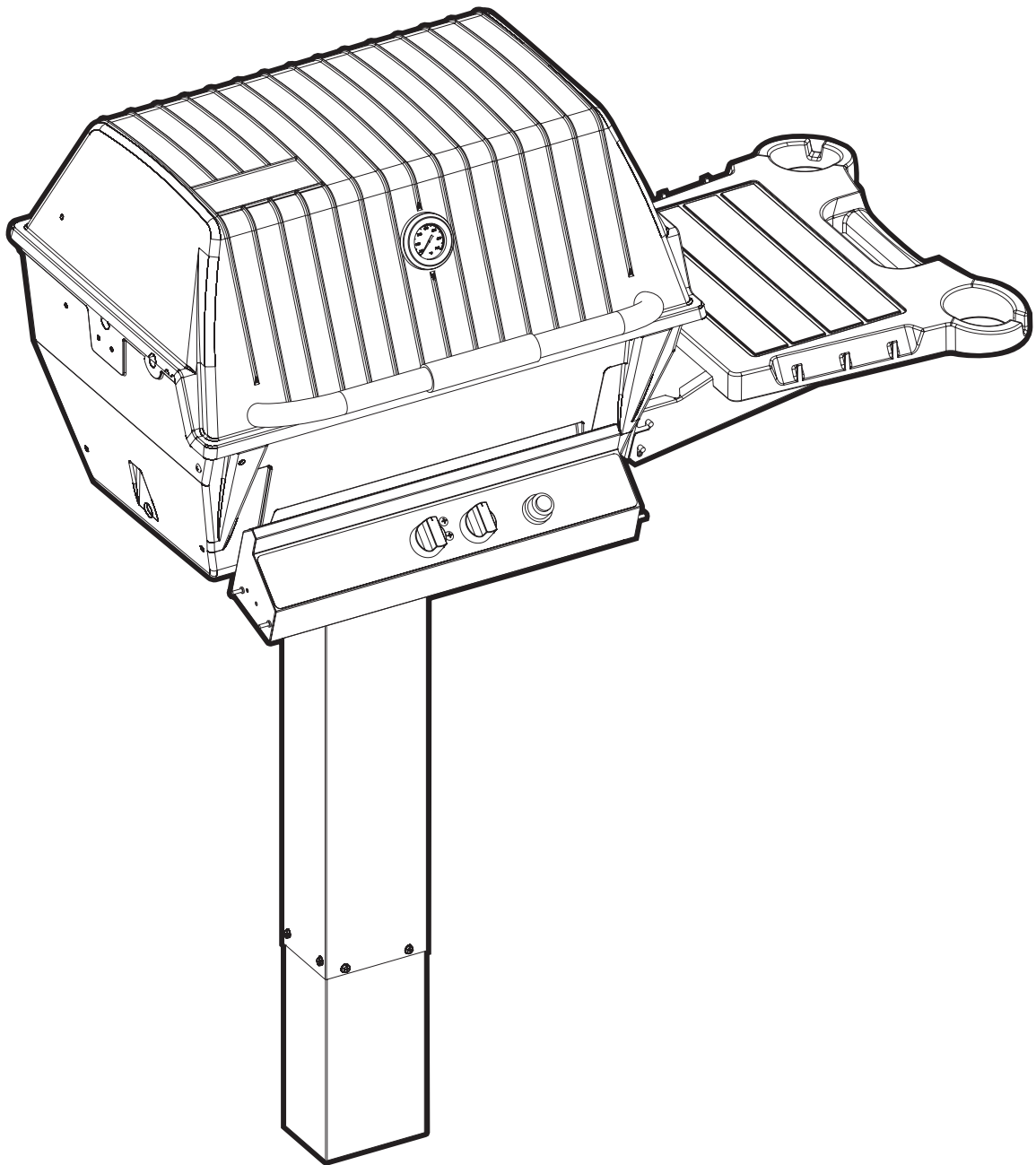
H3PK2N-3; H4PK2N-2; & H(3,4)PK2N-3 H(3,4)X GRILL WITH BLACK IN-GROUND POST AND ONE BLACK SHELF
